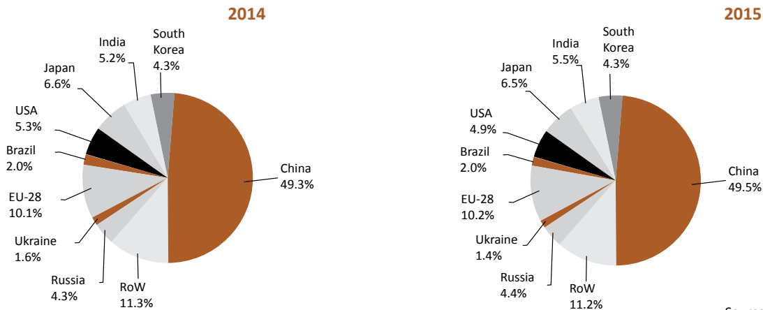
World Crude Steel production, 2014, 2015
