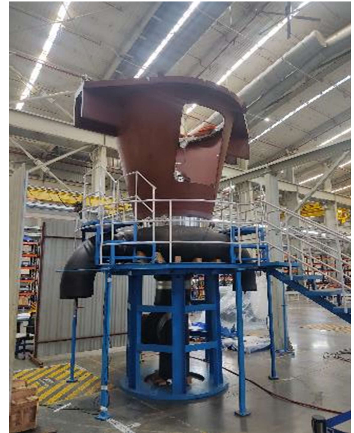
Hydro Test setup RSR 400
