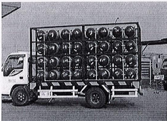
CNG Cascade with Type-IV Carbon Fibre Composite Cylinder
