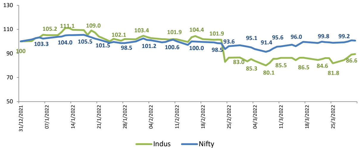
Nifty Comparison with Indus Tower (January 01, 2022 - March 31, 2022)
