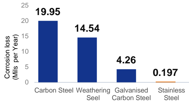
Corrosion resistance under wet /dry salt water environment
