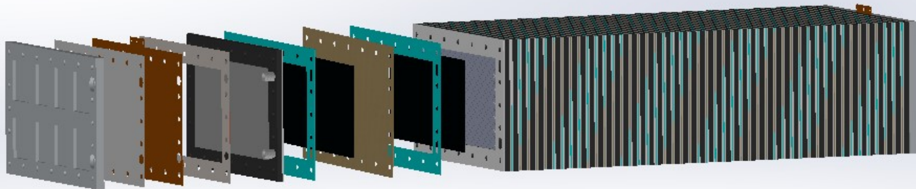
10 kW/50 kWh Containerized VRFB System
