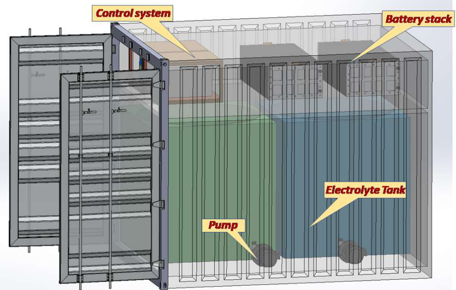
10 kW/50 kWh Containerized VRFB System
