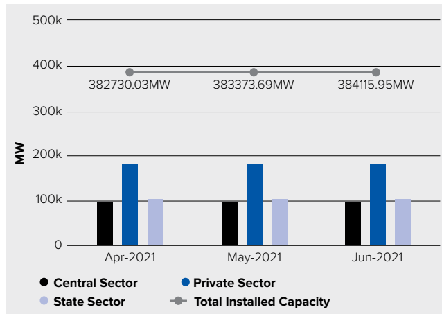
Figure 1: All India installed capacity (sector wise)
