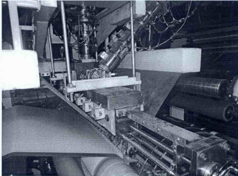
T-Die Section of the Extrusion Lamination Machine EL-1300 manufactured by Uflex Limited
