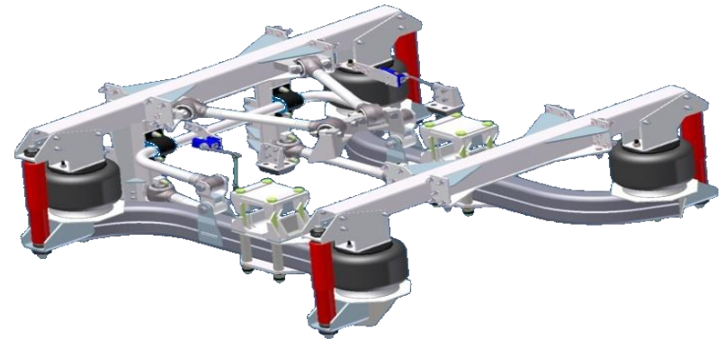
3) Air Suspension
